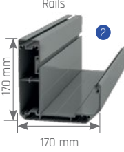
Extruded Frontal Gutter (Water-drain)
